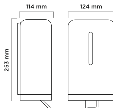
Cartridge Dimensions
