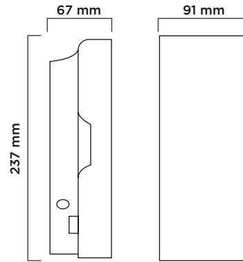
Cartridge Dimensions
