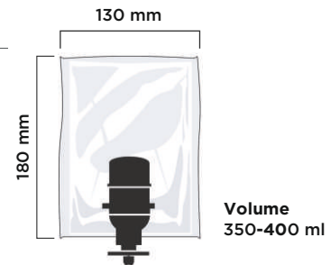
Cartridge Dimensions
